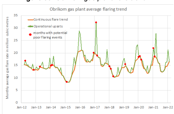
Figure 35: Obrikom gas plant flare trend
