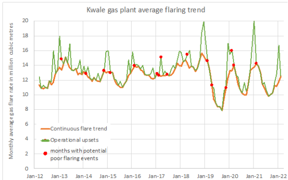
Figure 29: Kwale gas plant flare trend
