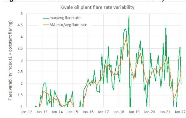
Figure 20: Kwale flow station flare rate variability
