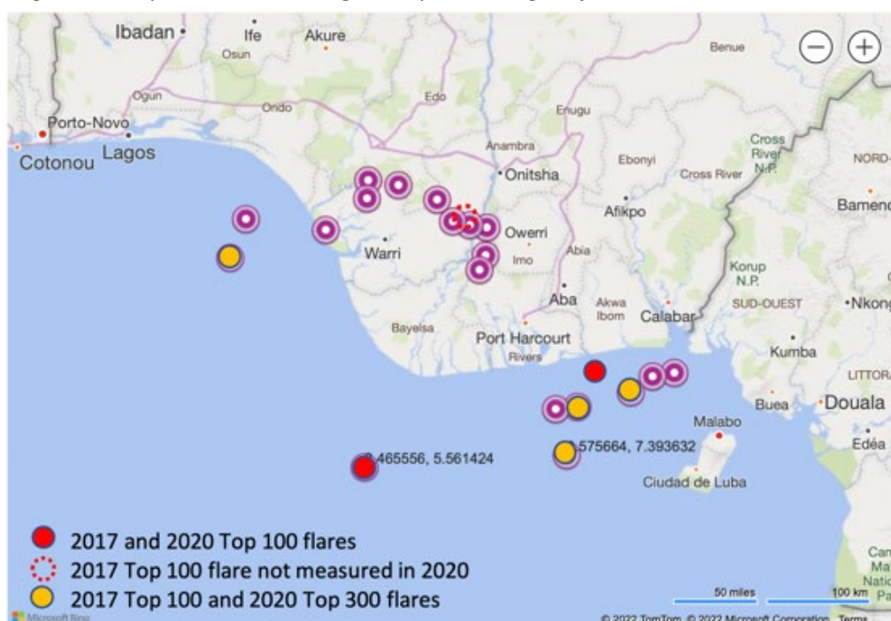
Figure 5: Nigeria's 20 super-emitter flares in global top 300 during the year 2020
