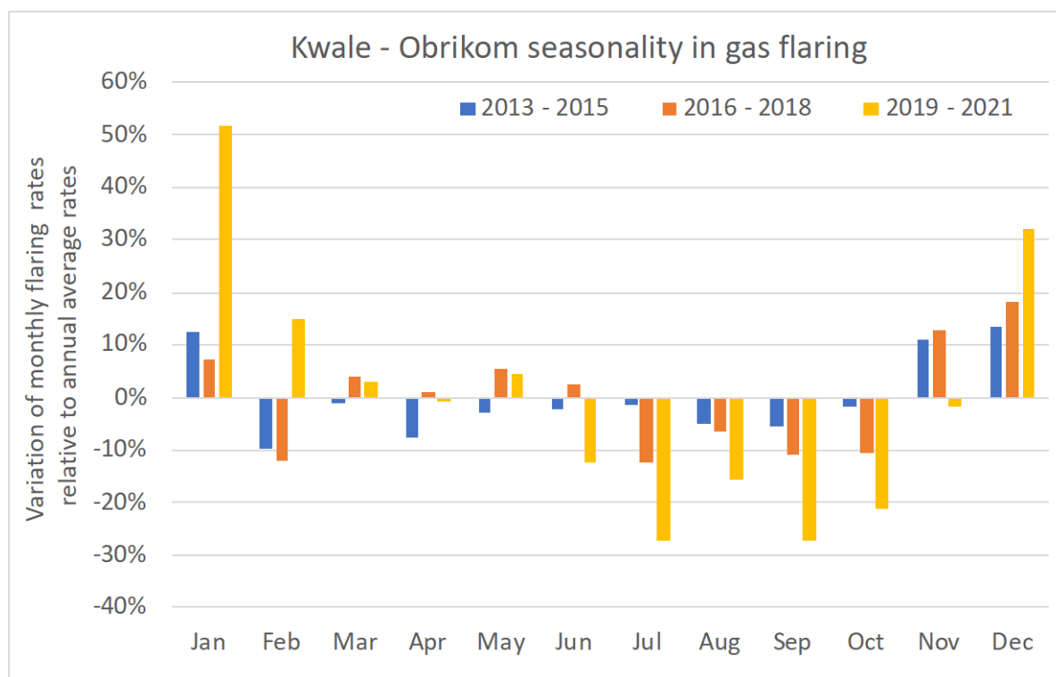
Figure 10: Seasonality in gas flaring of Ob-Ob and Kwale gas plants and Kwale and Ebendo flow stations
