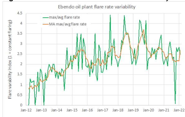
Figure 41: Ebendo flow station flare rate variability
