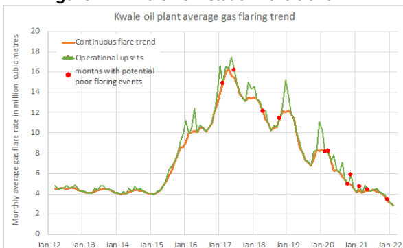
Figure 21: Kwale flow station flare trend
