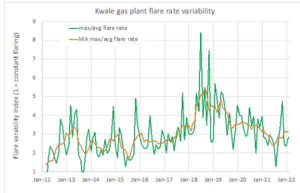
Figure 28: Kwale gas plant flare rate variability
