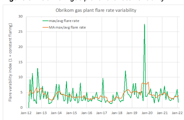
Figure 34: Obrikom gas plant flare rate variability
