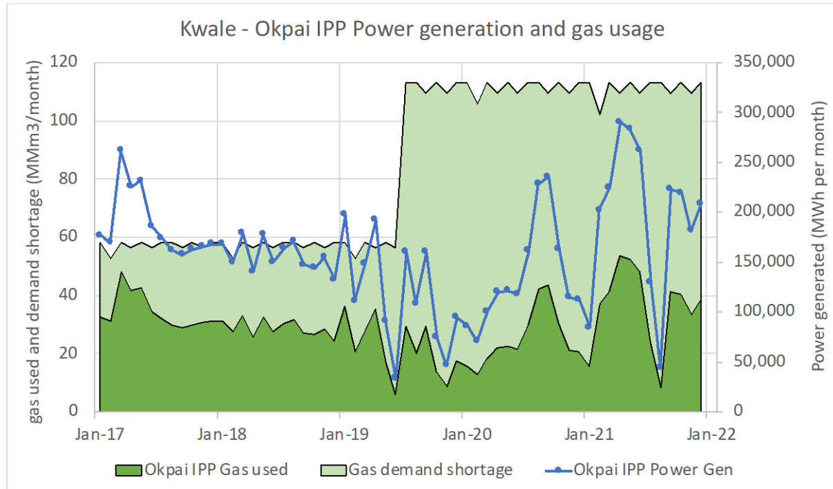
Figure 14: Kwale – Okpai IPP power generation and (shortfall) in gas demand
