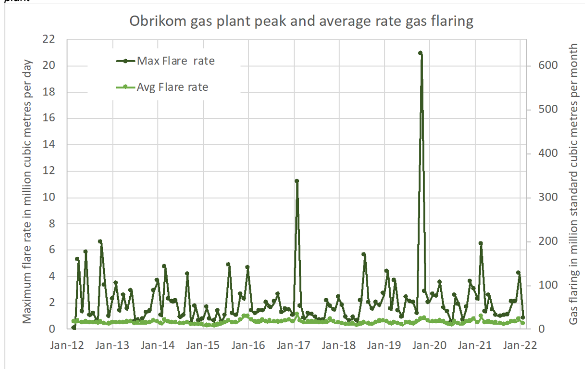
Figure 33: Monthly average and maximum daily peak flare rates of Obiafu-Obrikom (Ob-Ob) gas processing plant
