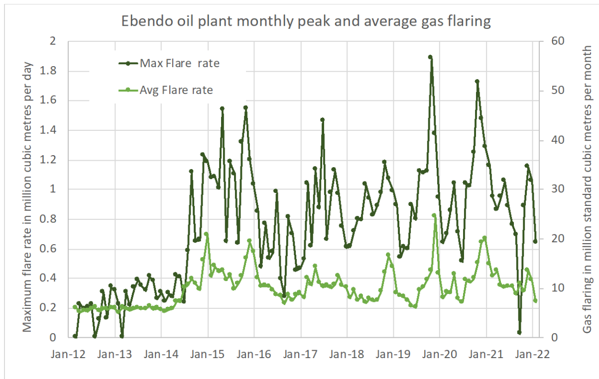
Figure 40: Monthly average and maximum daily peak flare rates of Ebendo flow station
