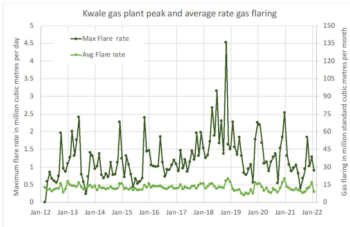
Figure 27: Monthly average and maximum daily peak flare rates of Kwale gas plant
