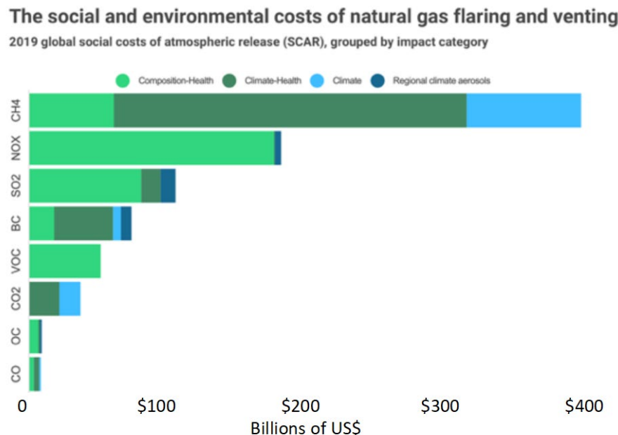
Figure 17: SCAR impact of global flaring and venting by individual chemical emitted
