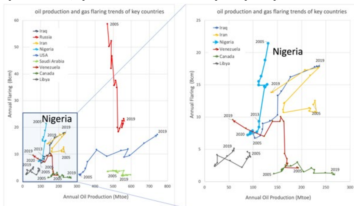
Figure 3: After Russia, Nigeria has been most successful in reducing natural gas flaring,
