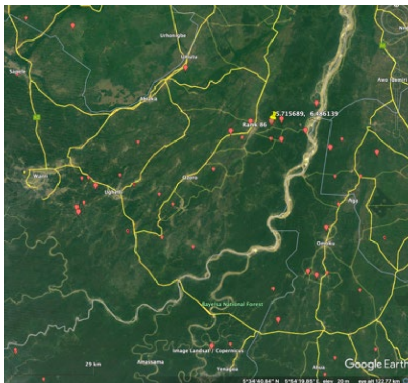
Figure 7b: In 2020, 62 flares in Warri area combust 234 MMscf/d gas, while the Kwale global super-emitter (indicated by the yellow pin) flared 9.2 MMscf/d.
