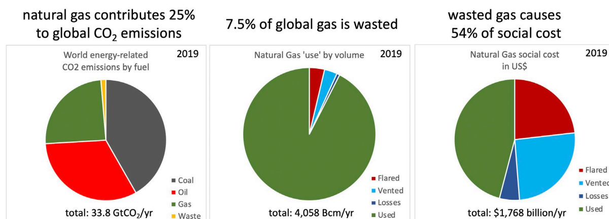
Figure 1: Natural gas flaring and venting has a disproportionately large impact on the social cost of the use of carbon energy.
