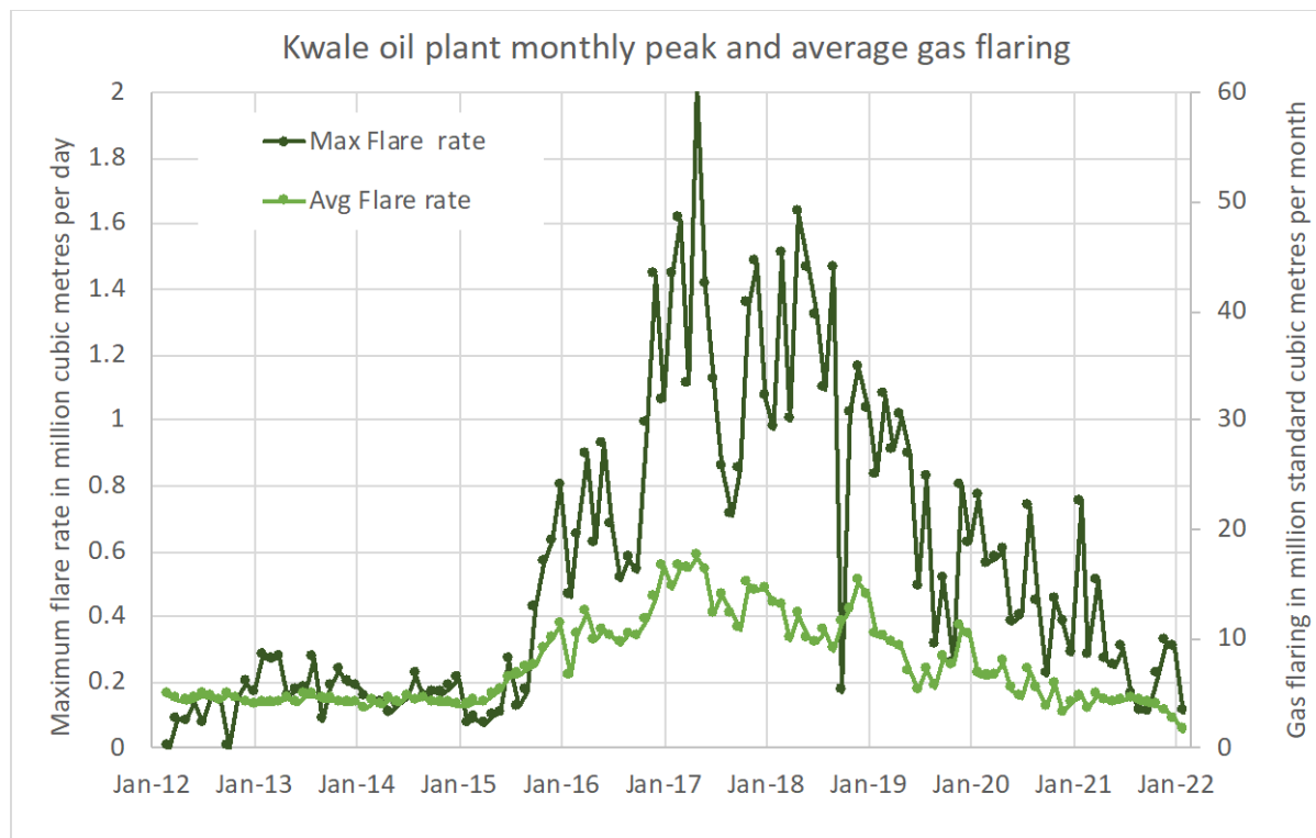
Figure 19: Monthly average and maximum daily peak flare rates for Kwale flow station
