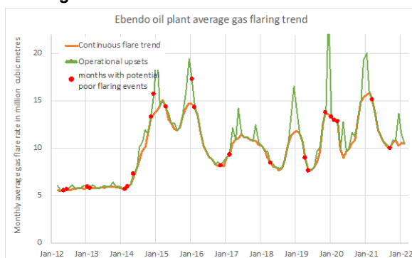
Figure 42: Ebendo flow station flare trend
